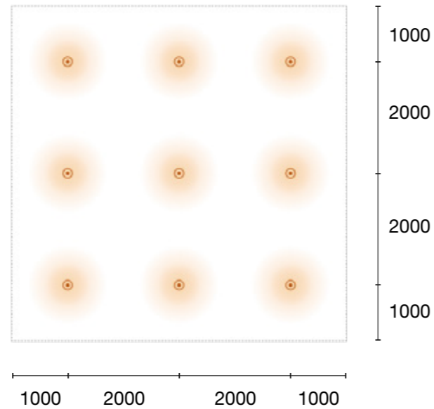
FLOOR LEVEL Target 160 lx @ 00 mm
