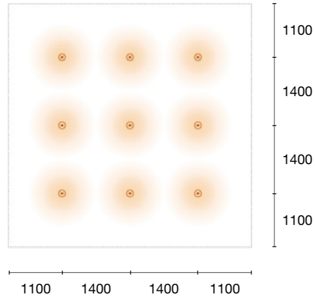
WORKSPACE Target 320 lx @ 750 mm
